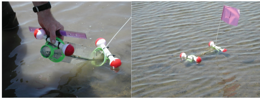
Fig. 5. Aquatic barrier trap used to sample rice water weevil adults and other aquatic.
